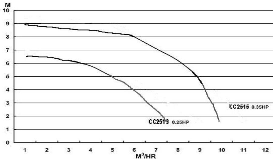
Pump Performance Curve
